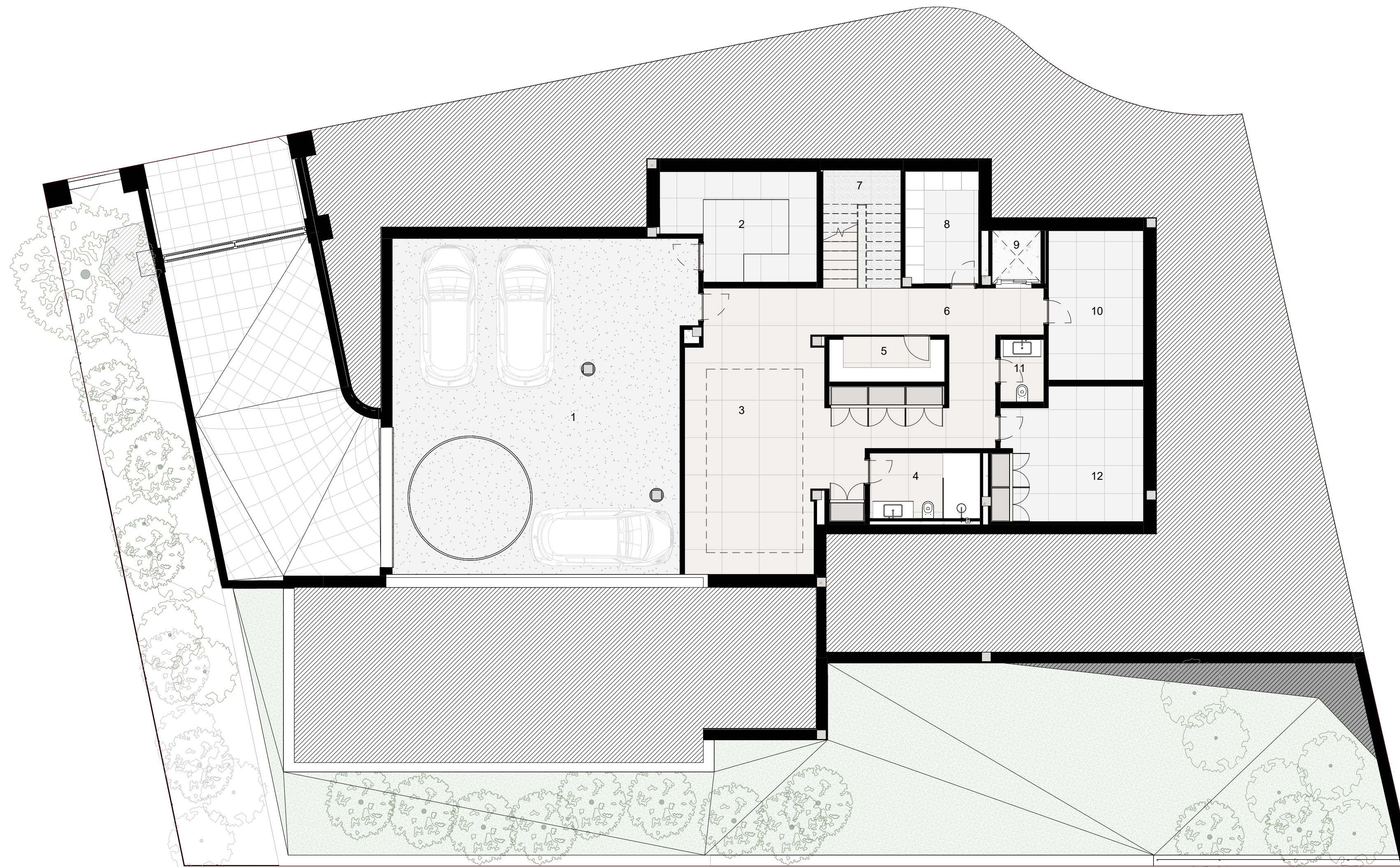
Basement floor
